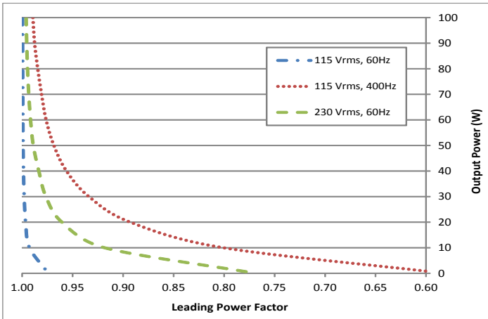
Figure 7: Output power vs. leading power factor (Tested with APFIC module and ACF-U-230-QM).
