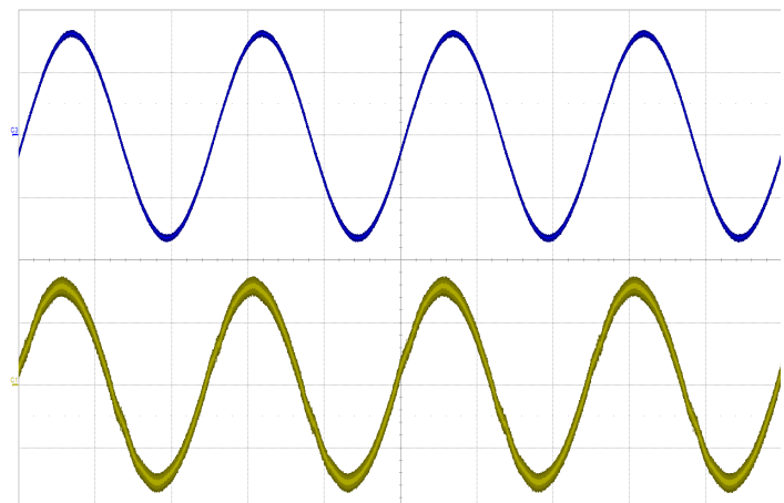
Figure 6: Typical Input Voltage and Current waveforms at full load current (115Vrms, 400Hz) Top: V_{in} (100V/div), Bottom: I_{in} (1A/div), Timebase: (1ms/div).
