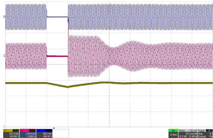
Figure 10: Line drop out with 400µF hold-up capacitor at full load current (115Vrms, 400Hz) Top: Vin (200V/div), Mid: Iin (2A/div), Bottom: Vout (20V/div), Timebase: (50ms/div).
