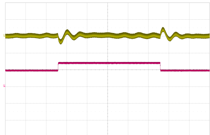
Figure 12: Regulated model output voltage response to step-change in load current with 200µF hold-up capacitor (50%-75%-50% of Iout(max), 115Vrms, 400Hz) Top: Vout (1V/div), Bottom: Iout (1A/div), Timebase: (100ms/div).
