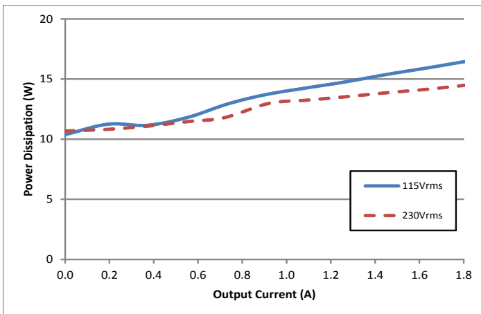
Figure 3: Power dissipation at nominal output voltage vs. output current for 115Vrms and 230Vrms (60Hz) input voltage at T_b = 25^\circ\text{C} .
