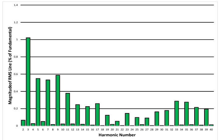
Figure 22: Input current harmonics at full Load, 115Vrms 400 Hz (Tested with APFIC module and ACF-U-230-QM).
