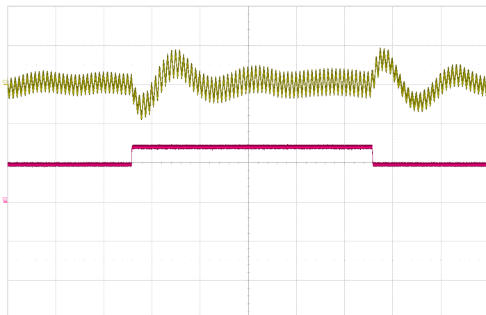
Figure 11: Regulated model output voltage response to step-change in load current with 200µF hold-up capacitor (50%-75%-50% of Iout(max), 115Vrms, 60Hz) Top: Vout (1V/div), Bottom: Iout (1A/div), Timebase: (100ms/div).
