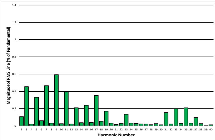
Figure 21: Input current harmonics at full load, 115Vrms 60 Hz (Tested with APFIC module and ACF-U-230-QM).
