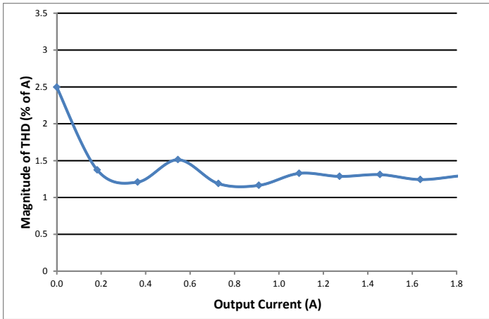
Figure 19: Total current harmonics at 60Hz, 115Vrms vs output current (Tested with APFIC module and ACF-U-230-QM).
