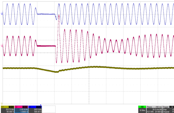
Figure 9: Line drop out with 400µF hold-up capacitor at full load current (115Vrms, 60Hz) Top: Vin (200V/div), Mid: Iin (2A/div), Bottom: Vout (20V/div), Timebase: (50ms/div).
