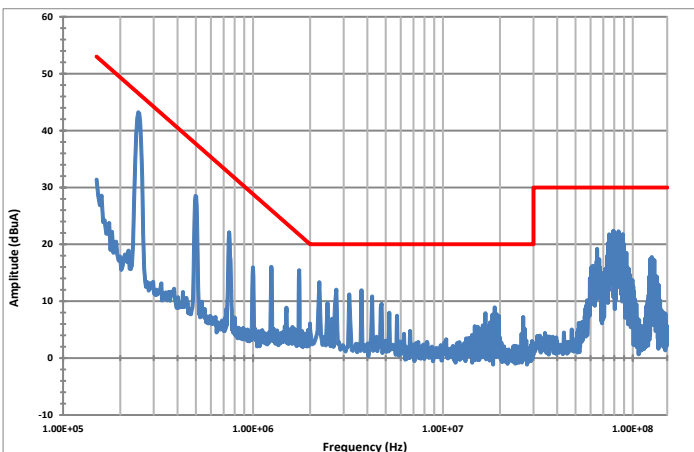
Figure 23: High frequency RTCA/DO-160G conducted emissions of ACF-U-230-QM filter and APFIC-U converter at full load, 115Vrms 60 Hz, category M limit. Preliminary.
