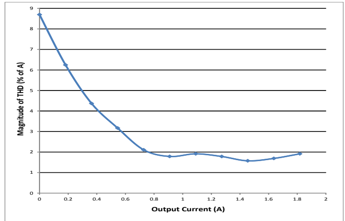
Figure 20: Total current harmonics at 400Hz, 115Vrms vs output current (Tested with APFIC module and ACF-U-230-QM).
