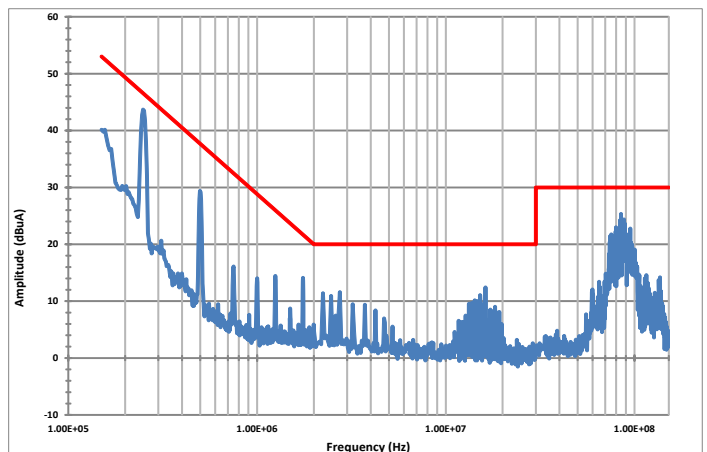
Figure 24: High frequency RTCA/DO-160G conducted emissions of ACF-U-230-QM filter and APFIC-U converter at full load, 115Vrms 400 Hz, category M limit. Preliminary.
