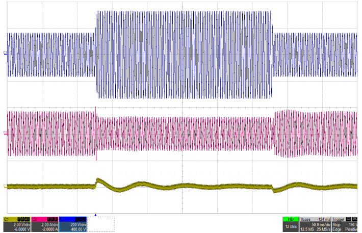
Figure 16: Input voltage transient response with 200µF hold-up capacitor at full load current (115Vrms-230Vrms-115Vrms, 400Hz), Top: Vin (200V/div), Mid: Iin (2A/div), Bottom: Vout (2V/div), Timebase: (50ms/div).
