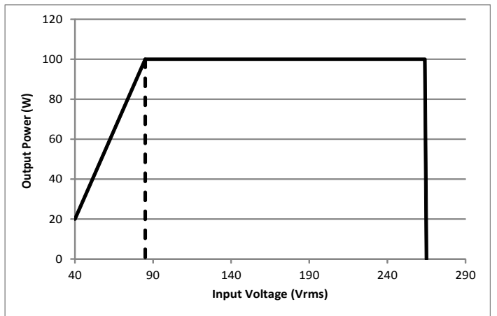
Figure 18: Maximum output power vs. input voltage, output turn-on threshold is 85Vrms.
