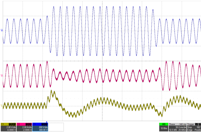
Figure 15: Input voltage transient response with 200µF hold-up capacitor at full load current (115Vrms-230Vrms-115Vrms, 60Hz), Top: Vin (200V/div), Mid: Iin (2A/div), Bottom: Vout (2V/div), Timebase: (50ms/div).
