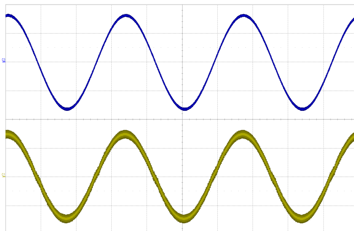
Figure 5: Typical Input Voltage and Current waveforms at full load current (115Vrms, 60Hz) Top: V_{in} (100V/div), Bottom: I_{in} (1A/div), Timebase: (5ms/div).
