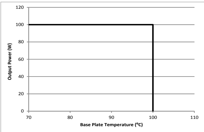
Figure 17: Maximum output power vs. base plate temperature derating curve.
